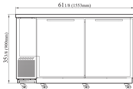
XBB-24-60SB-N6 FRONT VIEW
