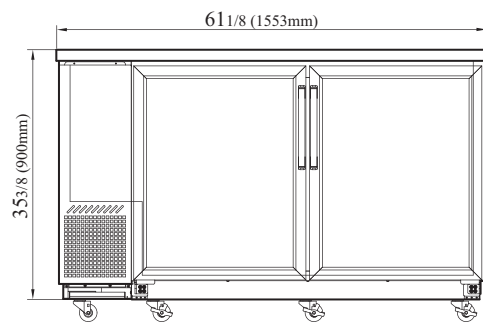
XBB-24-60SG-N6 FRONT VIEW
