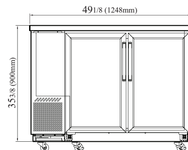
XBB-24-48SG-N6 FRONT VIEW
