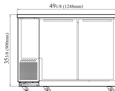
XBB-24-48SB-N6 FRONT VIEW
